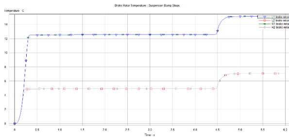
Figure28: Brake Rotor Temperature C-Time(s) "MAFSMC_ON"
