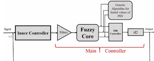
Figure8: Controller 2 scheme
