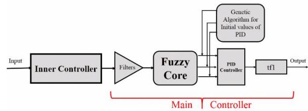
Figure7: Controller 1 scheme
